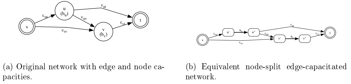
Figure 6.3: Node-splitting transformation.
